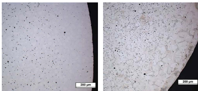
forMIM 316L.00 sintered unetched and etched microstructure at 7.9 g/cc density
